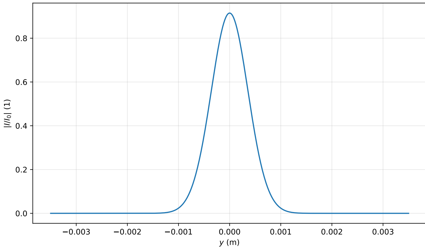
Intensity profile I(x=0, y, z=0.716)/I_0 , P_{in}=0.1P_{cr} , artificial time
